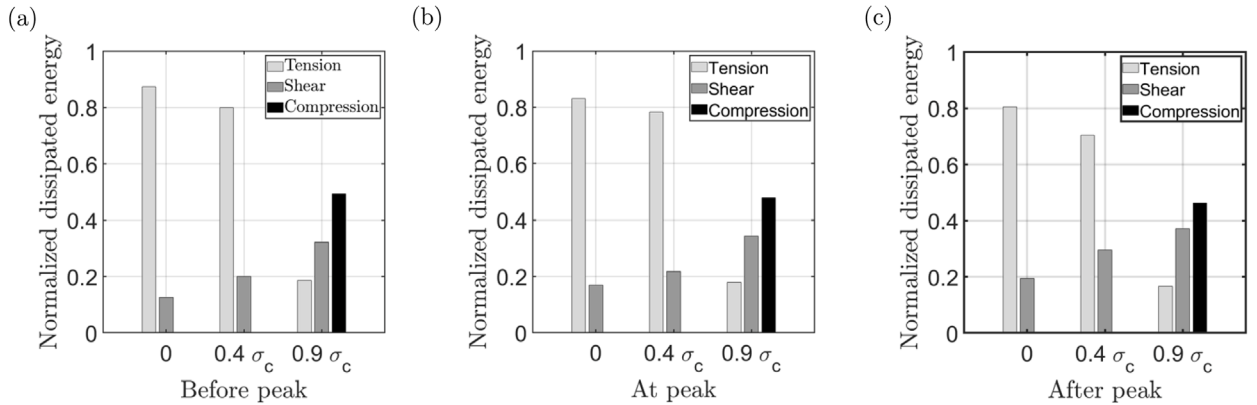
Fig. 12. Normalized dissipated energy for the medium samples with (a) 0\sigma_c , (b) 0.4\sigma_c , (b) 0.9\sigma_c .
