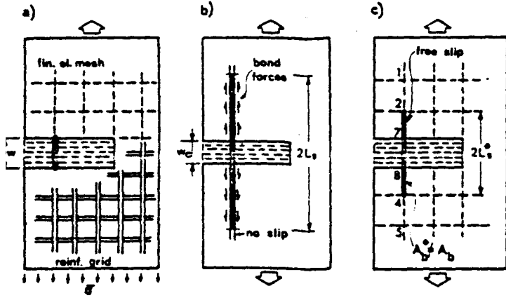
Fig. 9 - Illustrations of Bond Slip and Equivalent Free Bond Slip Length (after Bazant and Cedolin, 1980).
