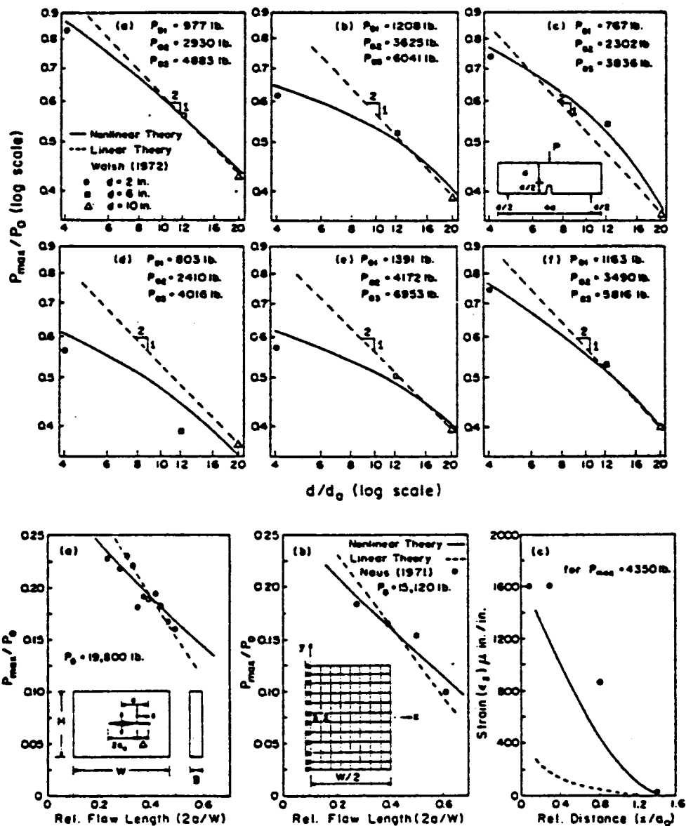
Fig. 5 - Results of Crack Band Analysis Compared With Maximum Load Test Data from the Literature (after Bazant and Oh, 1983).
