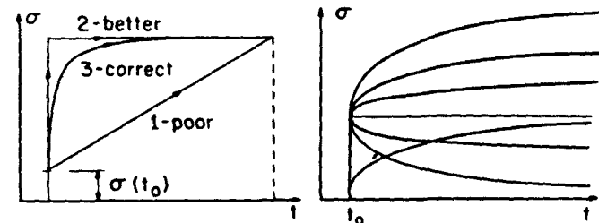
Figure 7.13 Strain histories expressed as a linear combination of the relaxation function
