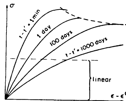
Figure 7.1 Creep isochrones
