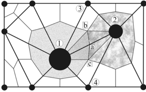
Figure 4. Example of two-dimensional tessellation of concrete mesostructure
