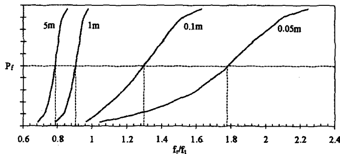
Figure 1. Cumulative probability distributions of modulus of rupture for different sizes.
