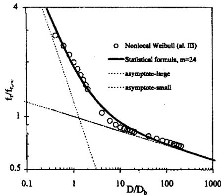
Figure 4. Optimum fit to the nonlocal Weibull theory.
