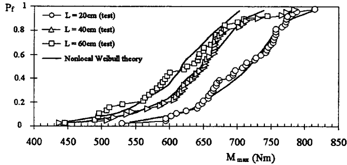
Figure 2. Comparison of CDF of maximum bending moment from Koide's (1998), series C, of four-point bending test and from the probabilistic nonlocal theory.
