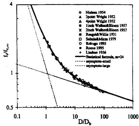
Figure 3. Optimum fit to existing test data.
