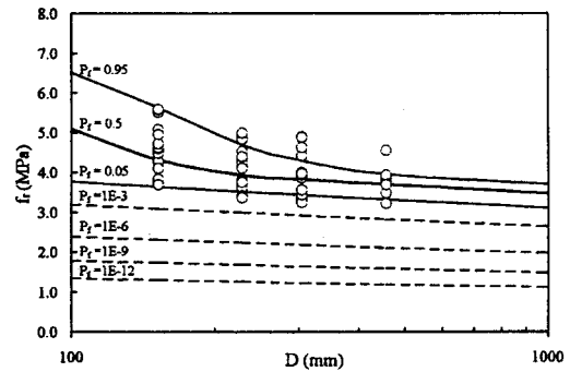
Figure 6. Failure probabilities vs. size for data of Lindner & Sprague (1956).
