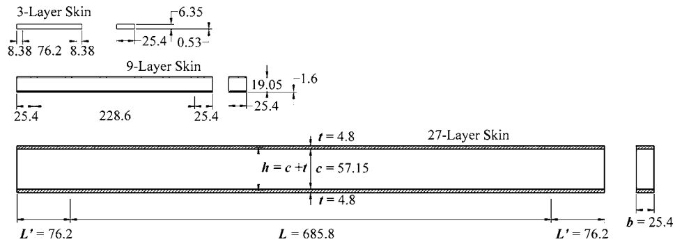
Fig. 7 Dimensions of test beams with no notches
