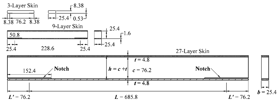
Fig. 4 Dimensions of test beams with notches at bottom
