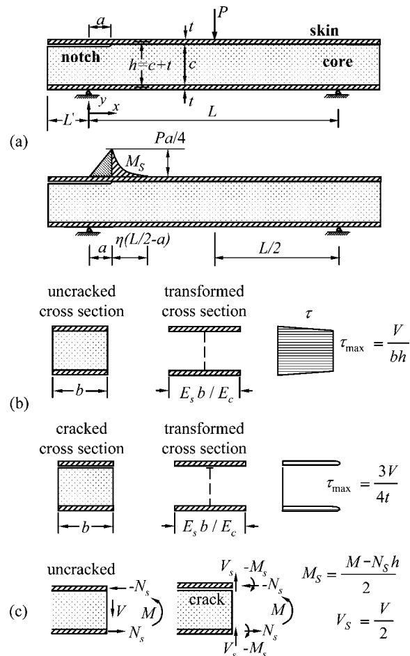
Fig. 11 Illustrations for beam-type analysis of fracture in the Appendix
