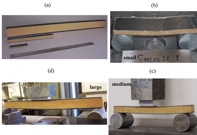
Fig. 8 (a) Photo of unnotched test beams of all three sizes; (b), (c), and (d) photo of typical failure modes for each of three beam sizes
