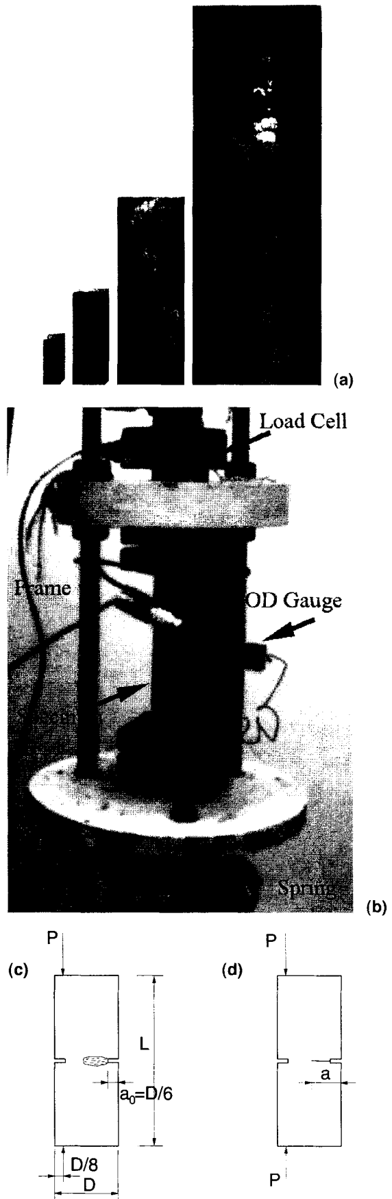
FIG. 1. Creep Specimens: (a) Edge-Notched Fracture Specimens Tested; (b) Instrumented Specimen in Loading Frame ( d = 3 in.); (c) Eccentric Compression Loading and Fracture Process Zone; and (d) Equivalent Crack of Length a
