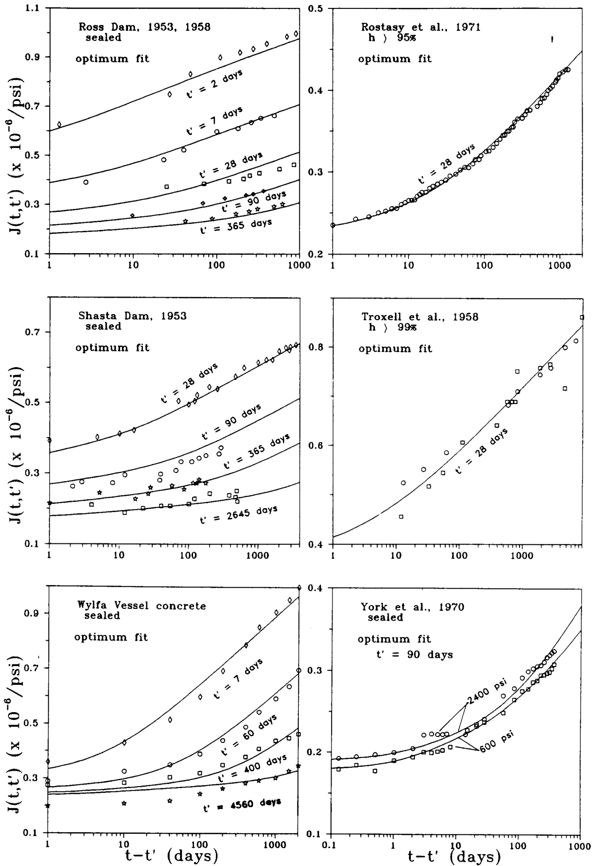
Fig. 7 Optimum fits of basic creep and data by Ross, Rostasy et al. , Hansen and Harboe (Shasta Dam), Browne and co-workers (Wylfa Vessel) and York et al. ; four parameters are optimized by linear regression.
