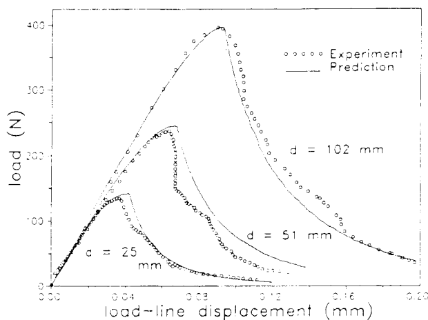
Fig. 14. Prediction of structural response.
