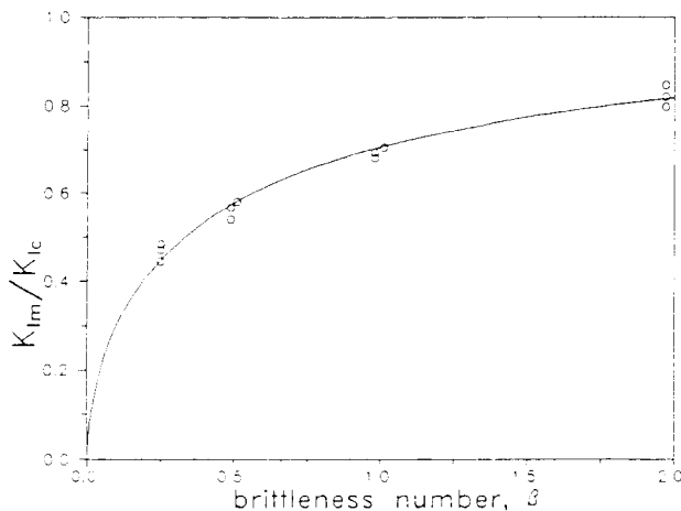
Fig. 11. Variation of apparent fracture toughness with size.
