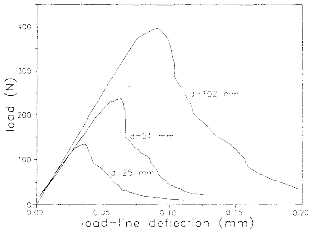
Fig. 7. Typical load-deflection curves.
