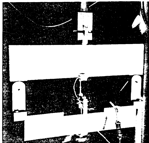
Fig. 6. Specimen test configuration.
