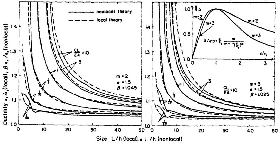
Fig. 5. Strain \epsilon_t at strain-localization instability (ductility) as a function of bar length L for various spring constants C and various shapes of stress-strain diagram ( m = 2 left, m = 3 right).
