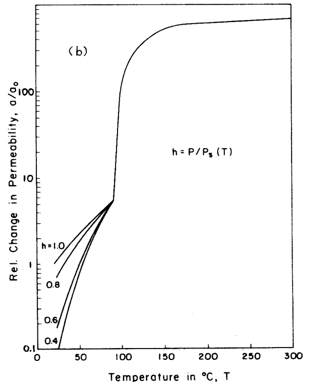
Fig. 1. (a) Sorption isotherms; (b) dependence of permeability on temperature and humidity.
