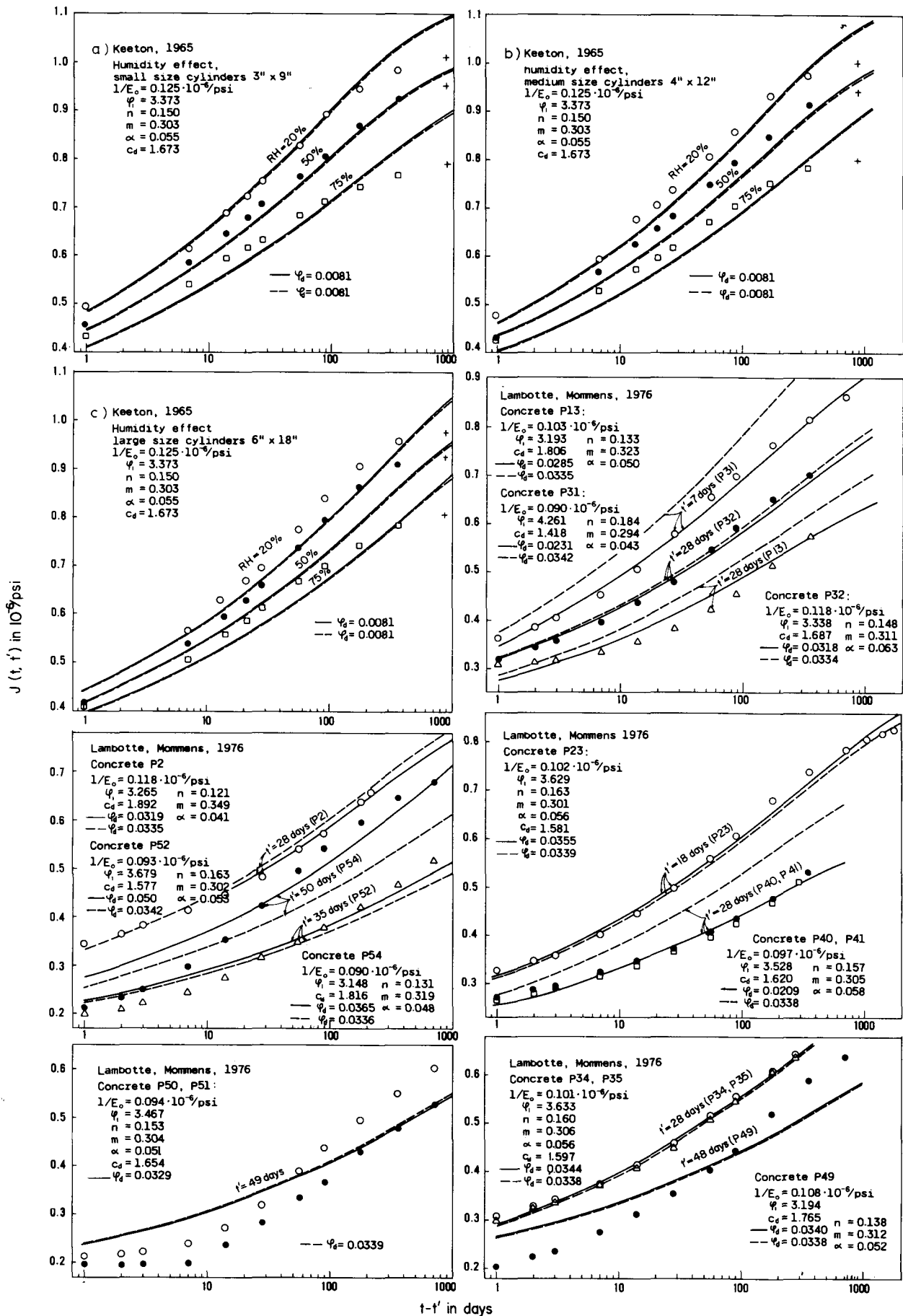
Fig. 20. — Fits of Tests for Drying Creep by Keeton (1965) [20] and Lambotte and Mommens (1976) [56]. \psi_d optimized — solid line, \psi_d by formula — dashed line. 1/E_0 calculated from experimental value E , if available, or optimized from basic creep data.
