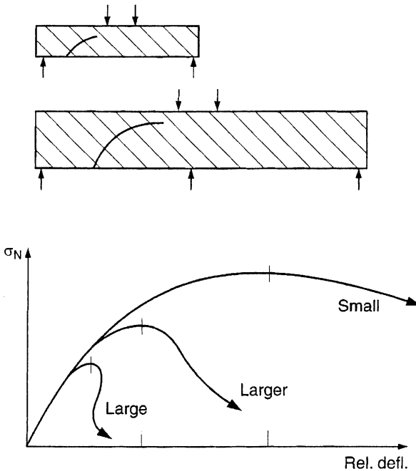
FIGURE 1.3.5 Load-deflection curves of quasi-brittle structures of different sizes, scaled to the same initial slope.
