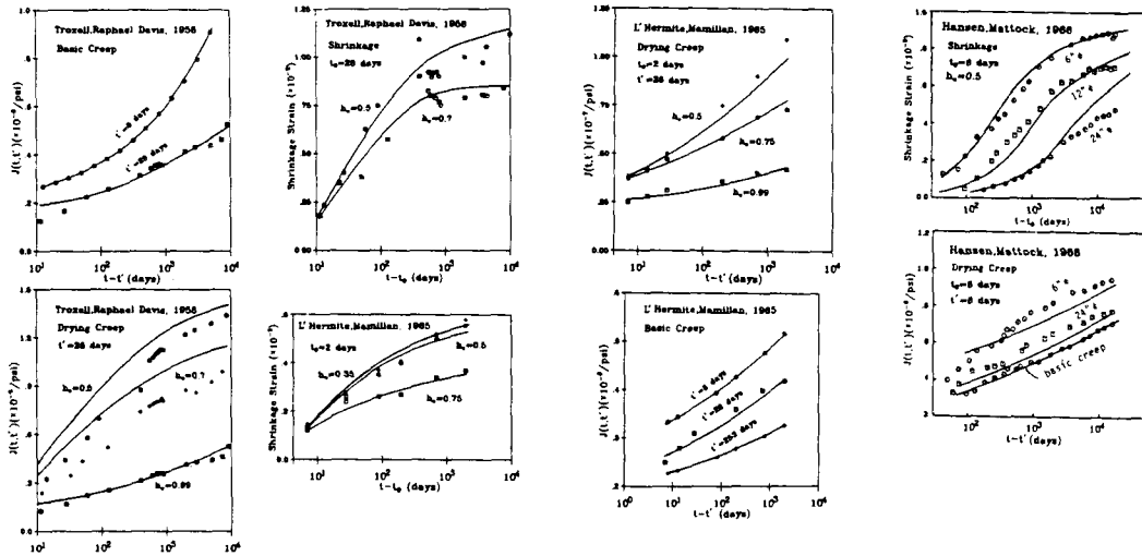
Fig. 3 - Stress-Induced Shrinkage Model with Cracking Compared with Previous Test Data (after Ref. 13).
