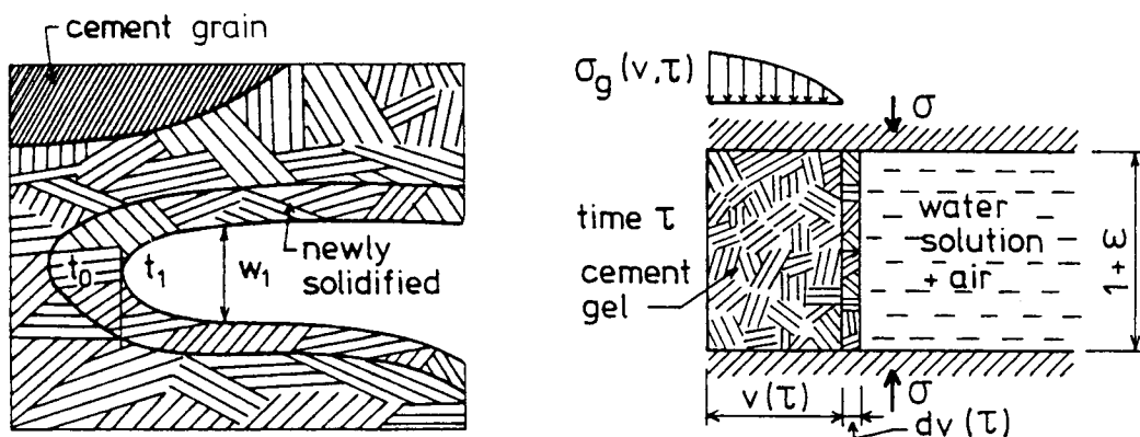
Fig. 2 - Model of Solidification of Portland Cement from Ref. 22.
