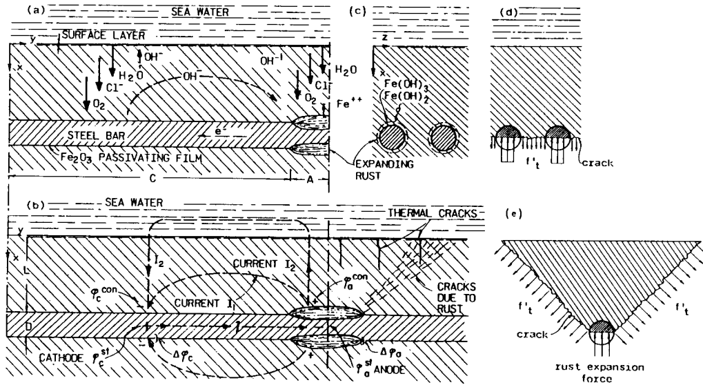
Fig. 5 - A simplified picture of the basic processes involved in steel corrosion and cracking of concrete cover (after Ref. 43).
