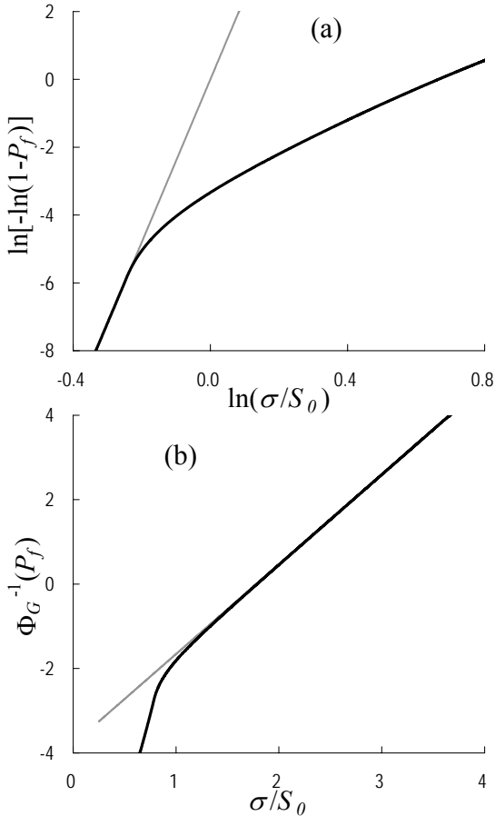
Fig. 3. cdf of a RVE with P_{gr} = 0.003 and CoV = 25\% in a) Weibull probability paper; b) normal probability paper
