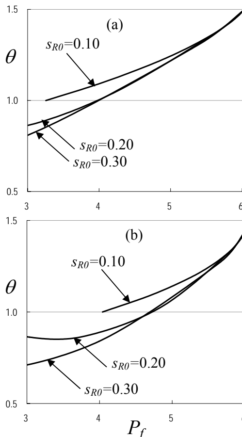
Fig. 6. Ratios \theta calculated for coefficient of variation of load: a) s_L=0.10 ; b) s_L=0.20 .
