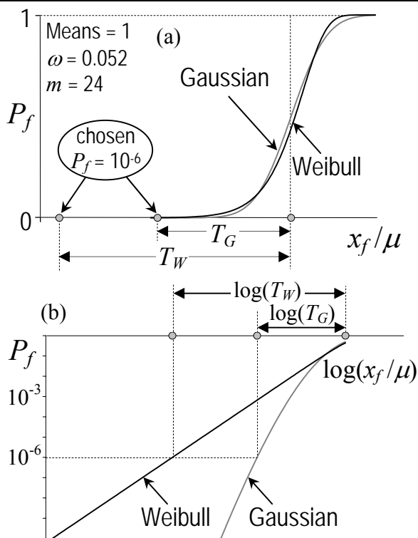
Fig. 5. Large difference between points of failure probability 10^{-6} for Gaussian and Weibull distributions with mean 1 and CoV = 5.2% in (a) linear scale; (b) log scale.
