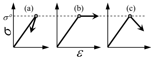
Fig. 2. Post-peak behaviour of fibers: a) Brittle; b) Plastic; c) Elastic Softening
