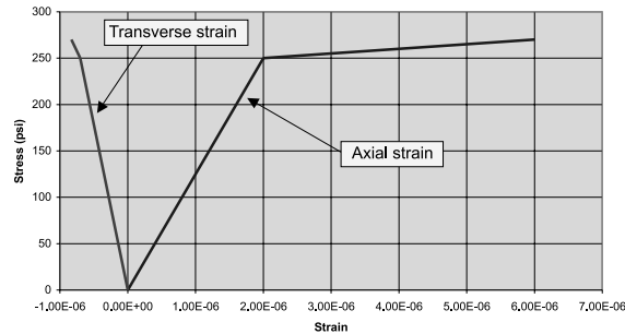
Fig. 7. Axial and transverse strain in uniaxial compression test beyond the yield point, predicted by the microplane model (the compressive strain and stress are plotted as positive).
