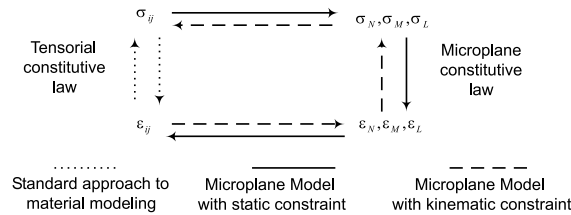
Fig. 3. Patterns for stress or strain update in the microplane model with static or kinematic constraint.
