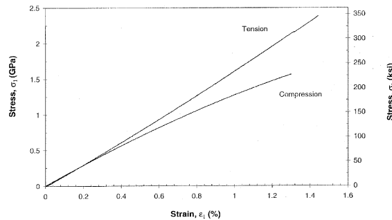
Fig. 12. Longitudinal tensile and compressive stress–strain behavior of AS-4/3501-6 unidirectional carbon-epoxy composite.
