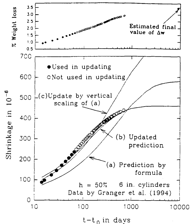
Fig. 4 Updating of shrinkage prediction using short term test data. Data by Granger [38].
