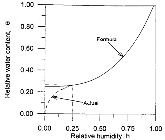
Fig. 3 Relative water content, \theta = 1 - \Delta w_x(h)/\Delta w_x(0) , versus relative humidity h .
