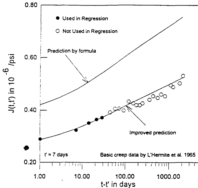
Fig. 1 Example of improving the prediction of creep by the use of short term test data. Basic creep data by L'Hermite et al. [14].
