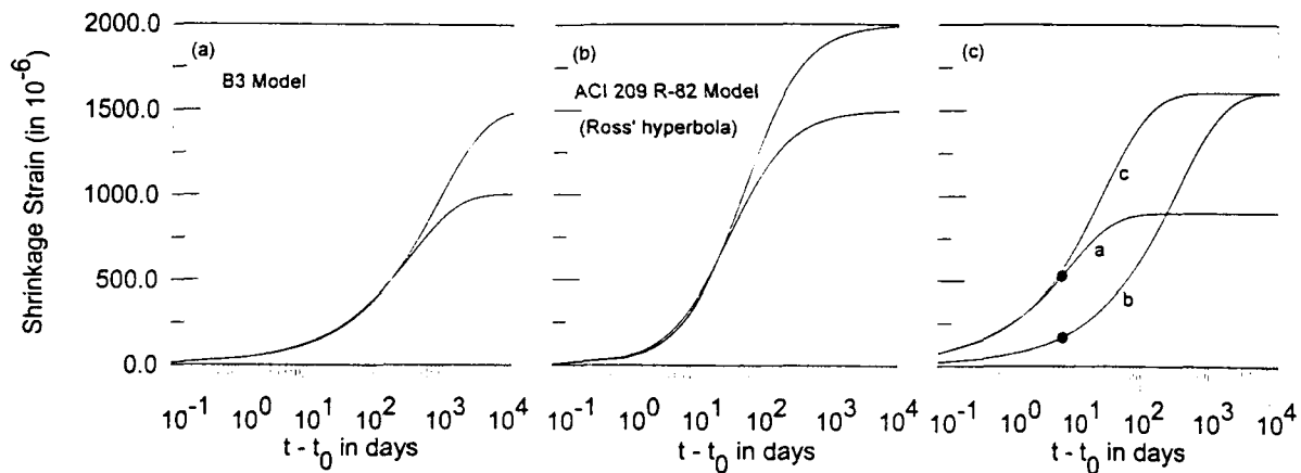
Fig. 2 (a, b) Example of shrinkage-time curves giving nearly the same development of shrinkage for short times but very different final values, and (c) possible shrinkage curves of identical specimens of different concretes.
