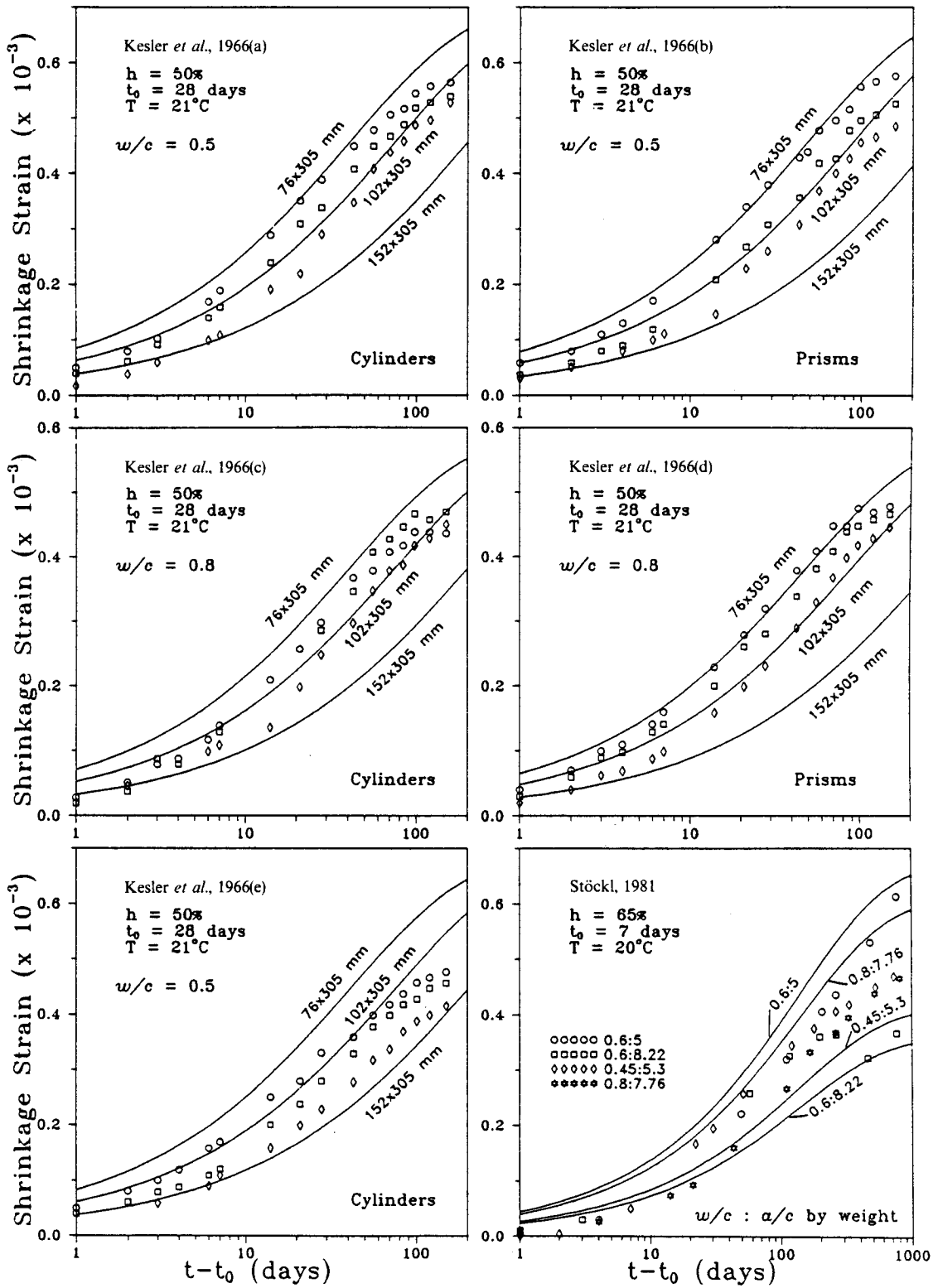
Fig. 4 Predictions of shrinkage and data by Kesler et al. and Stöckl.
