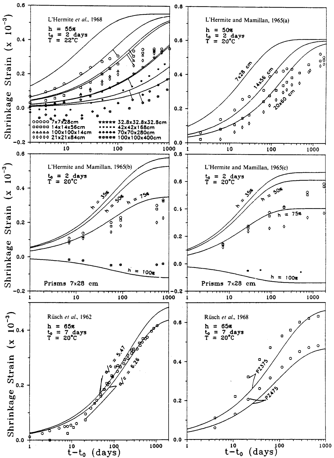
Fig. 5 Predictions of shrinkage and data by L'Hermite et al. , L'Hermite and Mamillan and Rüsç et al.
