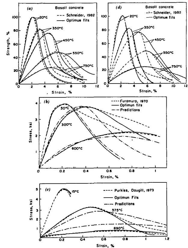
FIG. 4. (a) Schneider's (18) Tests at Constant Stress Rate and Various Temperatures; (b) Compression Stress-Strain Curves Measured by Furumura (19); (c) Compression Stress-Strain Curves Measured by Purkiss (20); (d) Predictions of Concrete Response for Schneider's Tests
